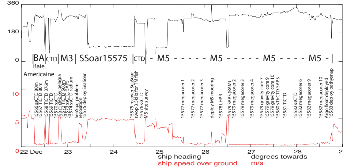
Fig. 1.3.7a - D286 week 2 22-28 Dec wind, irradiance, pressure, ship speed, direction
