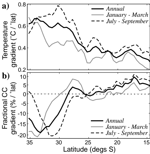
Figure 3: Mean meridional gradients between 50°E and 105°E. a) SST (in degs C per degree of latitude), b) Chlorophyll concentration (percentage change per degree of latitude).
