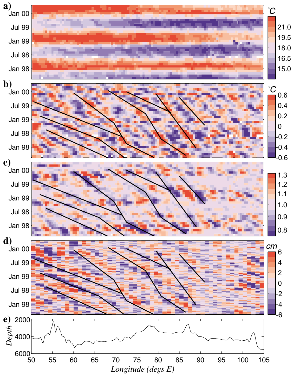
Figure 1: Hovmöller diagrams at 34°S in the Indian Ocean of various water properties. a) SST, b) SST anomalies, c) CC anomalies, d) SSH anomalies (see text for further details). e) Bathymetry for the section. [ The solid lines are discussed in section 3a. ]
